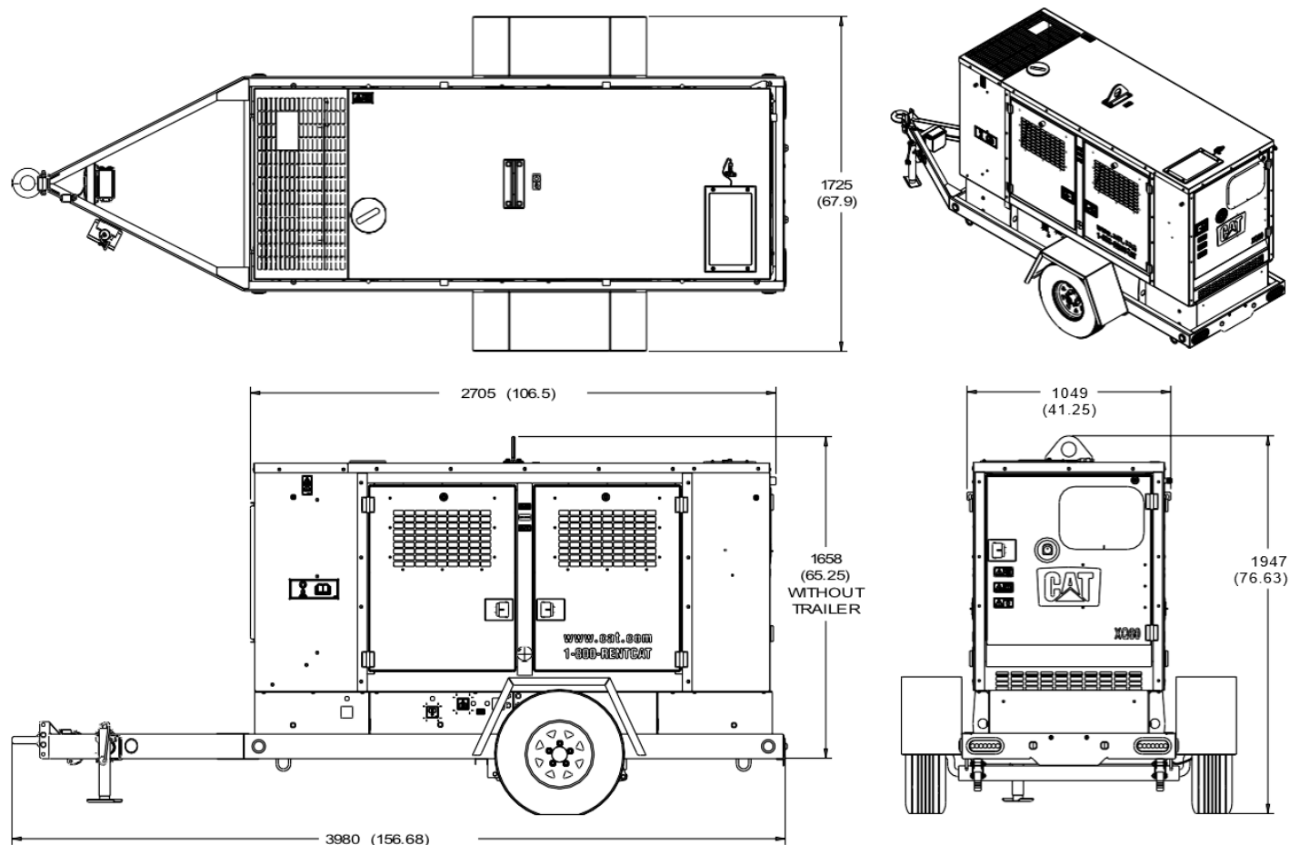
XQ60 GENERAL LAYOUT DRAWING
