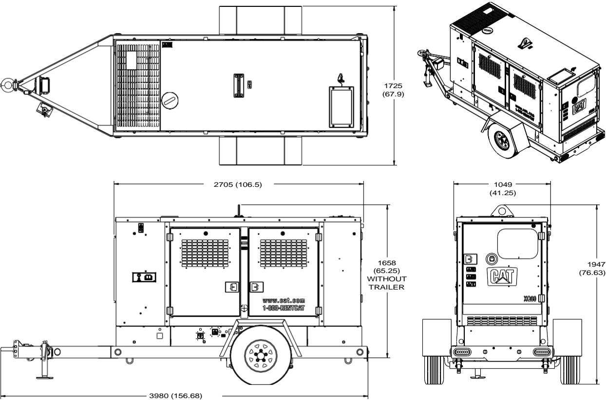
XQ60 GENERAL LAYOUT DRAWING
