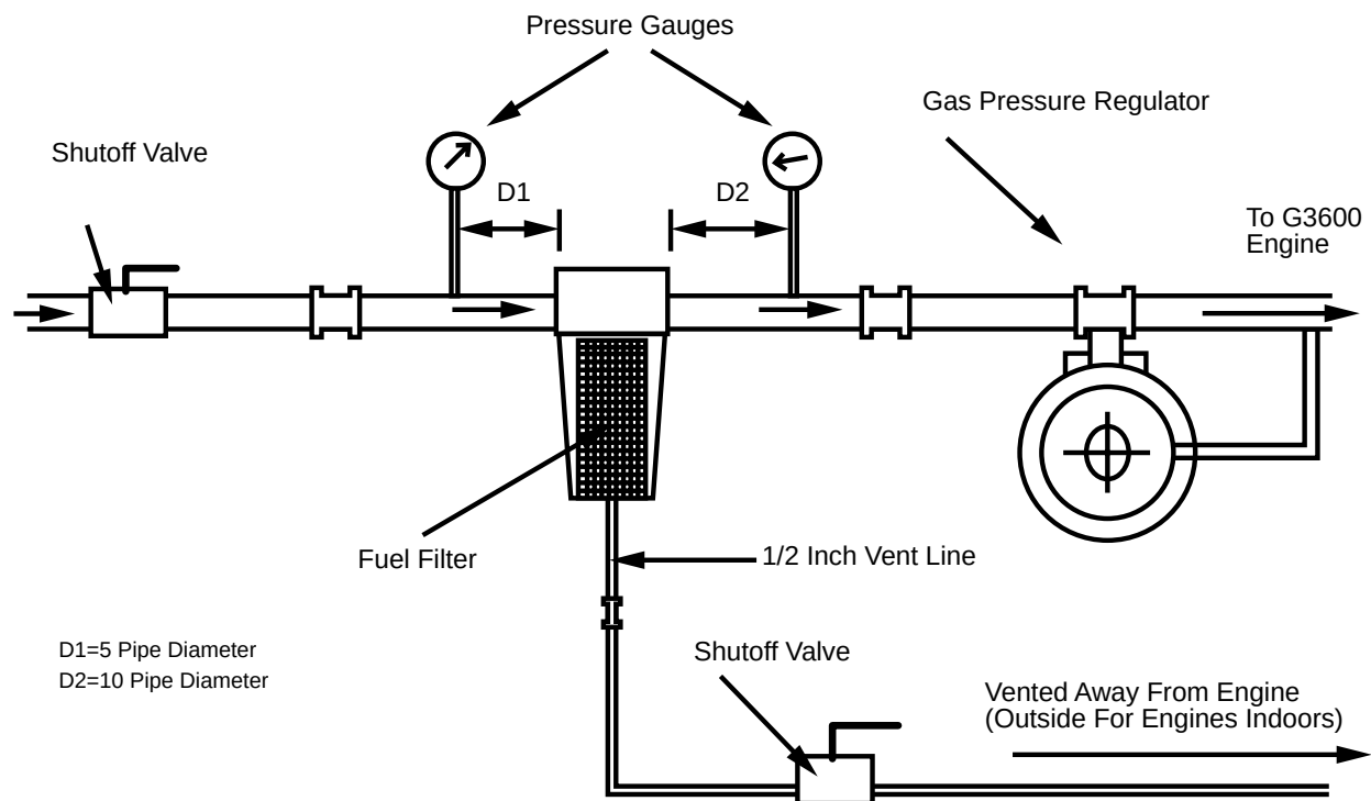
Figure 1. Fuel Filter connections.
