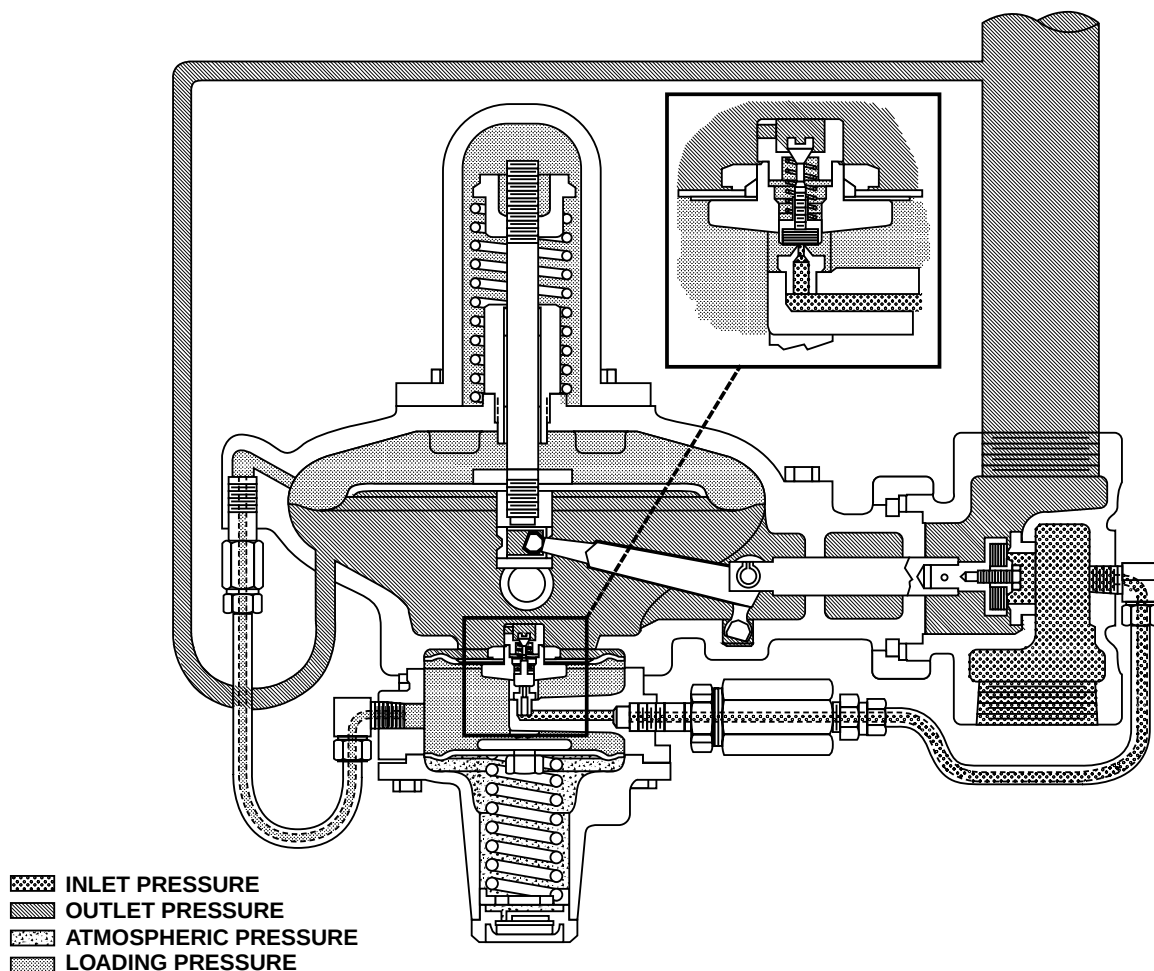
Figure 2. Regulator Schematic.
