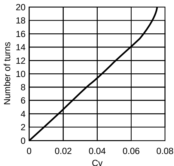
Figure 4. Flow vs. Number of turns.
