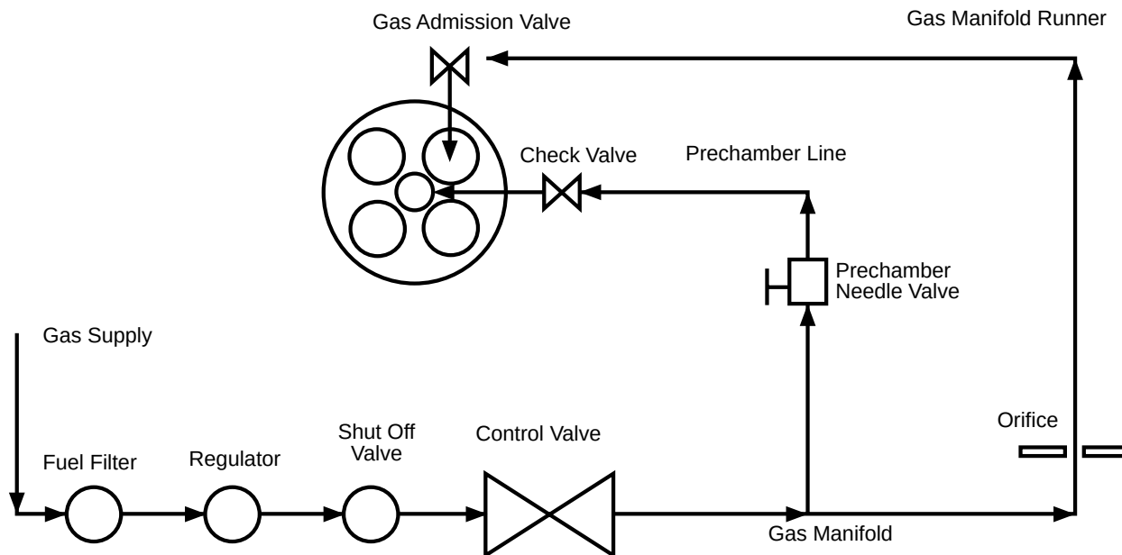
Figure 3. Fuel System Schematic.
